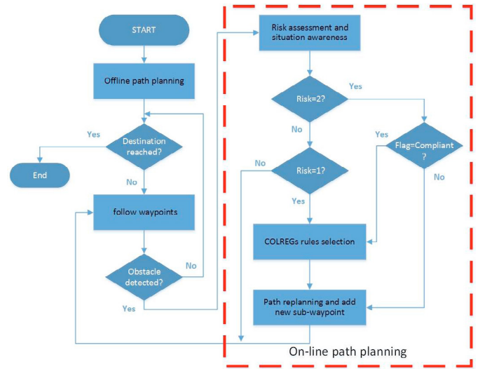
Fig. 3. Flowchart of the path planning process
