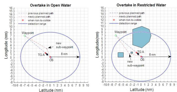
Fig. 4. Overtaking in open water and restricted water
